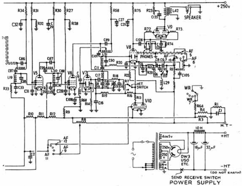
Fig. 2. Circuit of modified R1155 Receiver.
